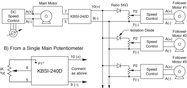
FIGURE 5 – LEADER/MULTIPLE FOLLOWER VOLTAGE FOLLOWING SYSTEM
